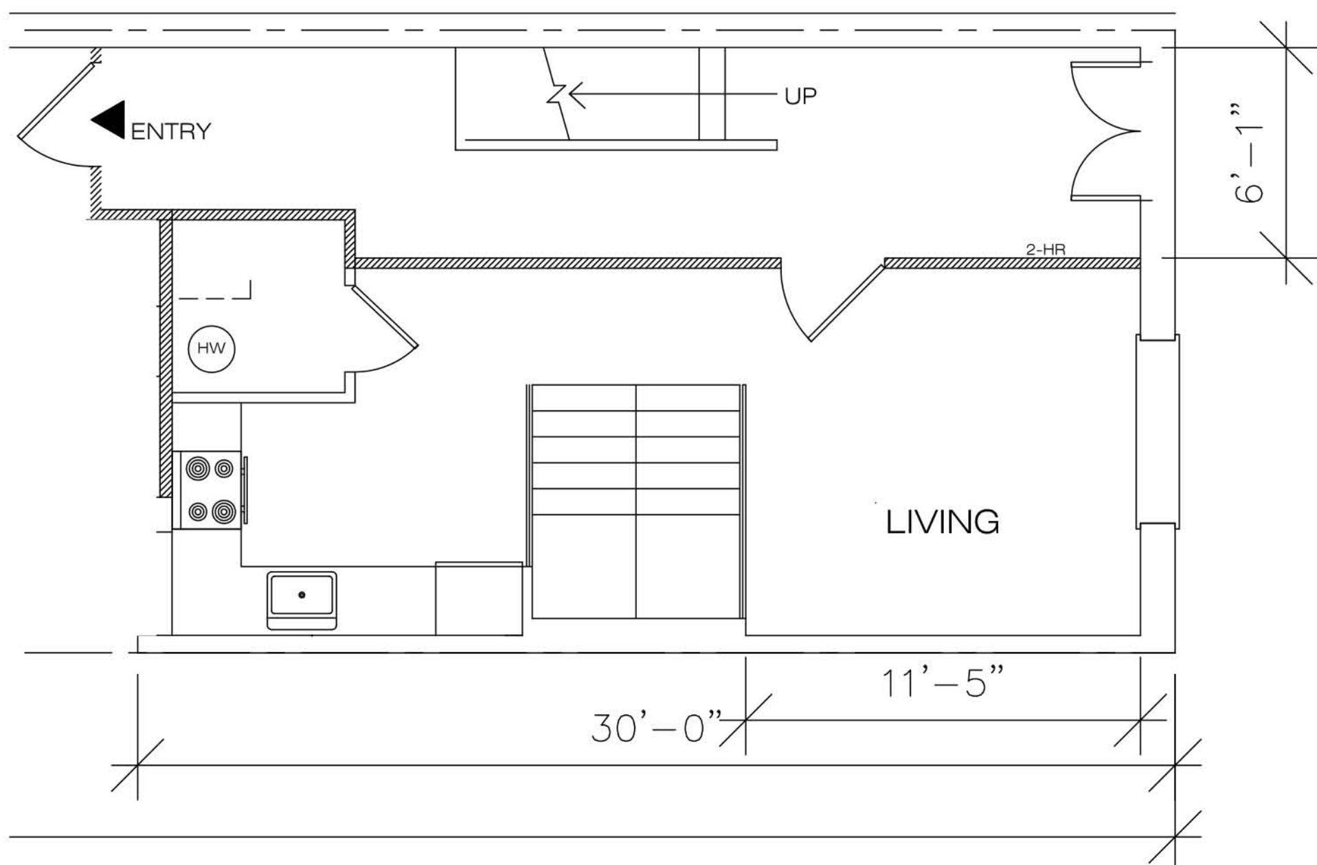
1st floor level
