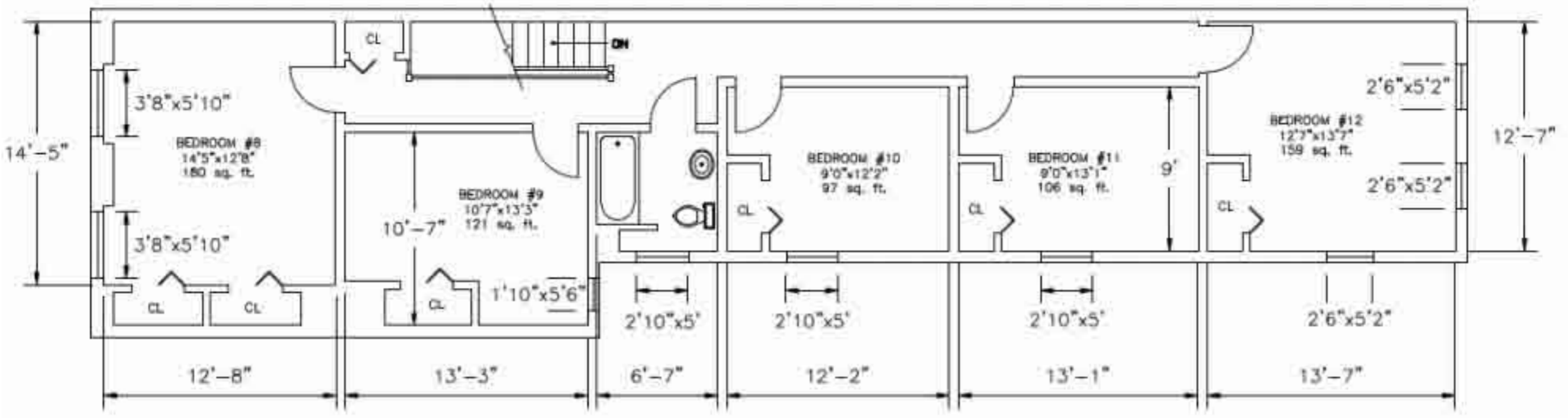
Third Floor Scale: 3/32" = 1'-0"
