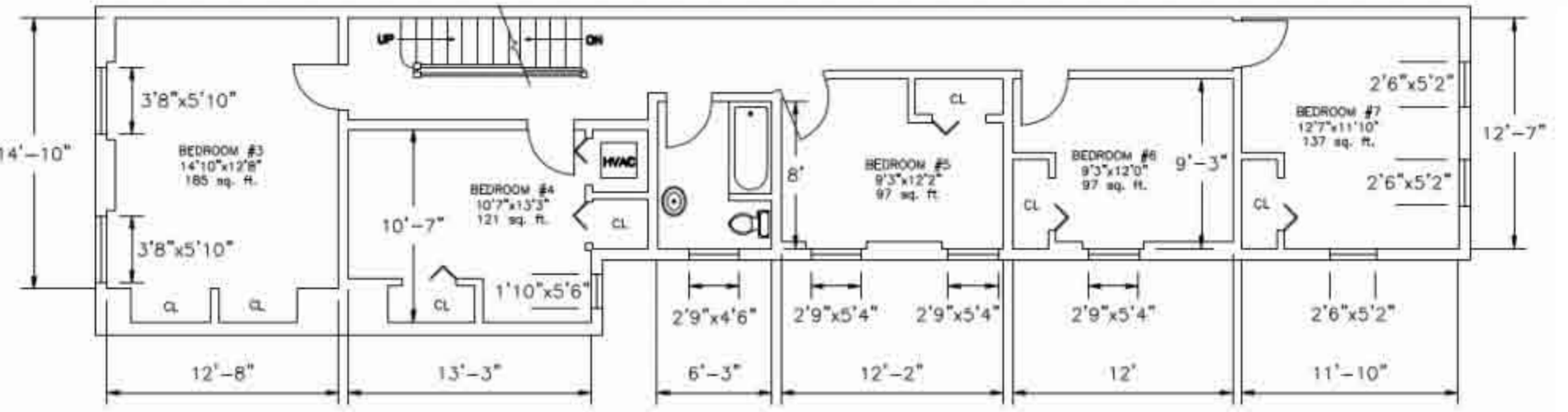
Second Floor Scale: 3/32" = 1'-0"
