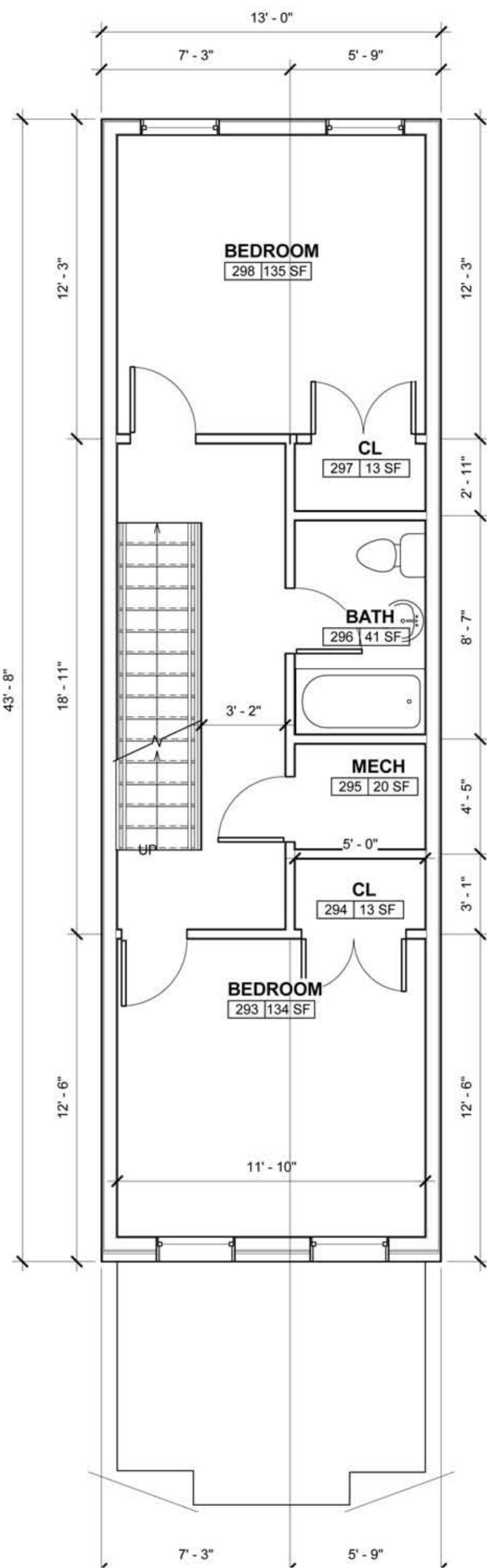
3rd Floor
