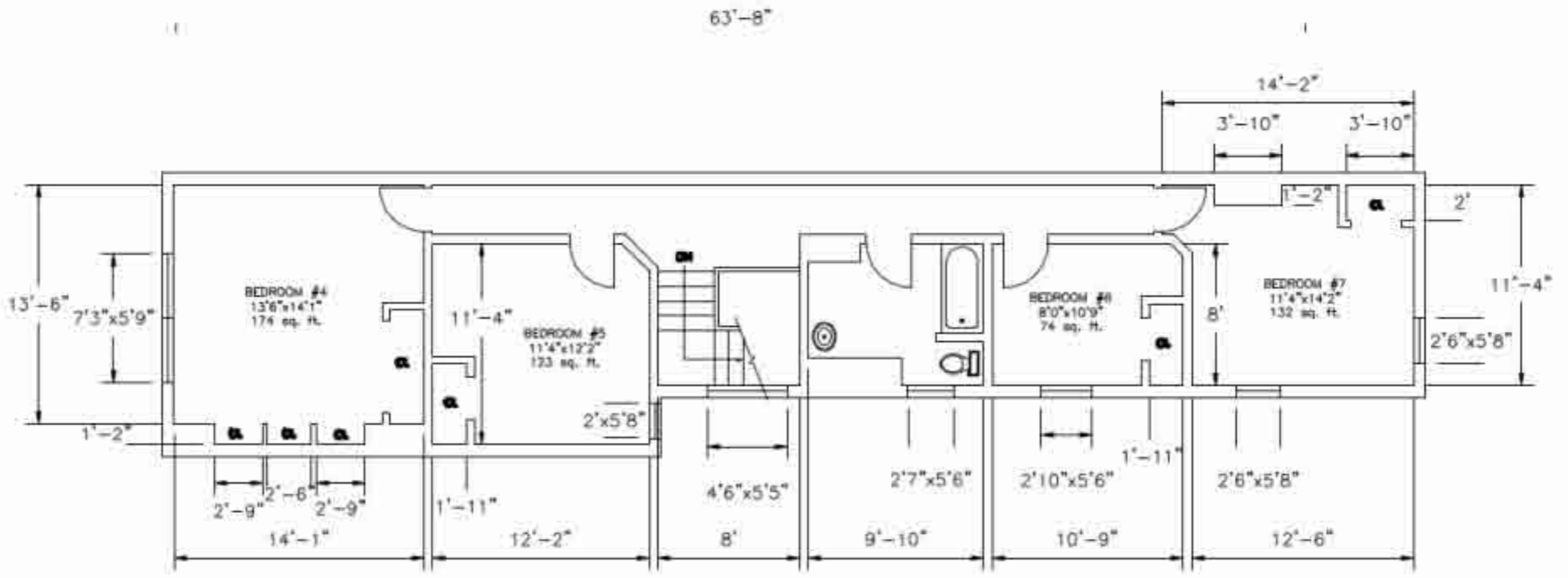
Third Floor Scale: 3/32" = 1'-0"
